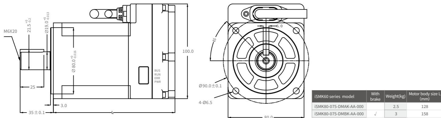
iSMK80 series mechanical dimension diagram (unit: mm)
