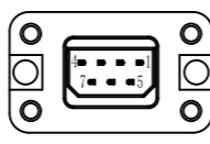
Encoder socket multiturn
