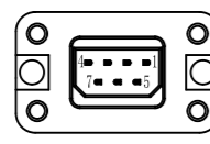
Encoder socket single turn
