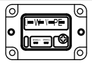
SMK60 power socket without brake
